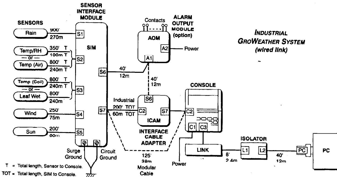
Figure 1a. GroWeather System Schematic
