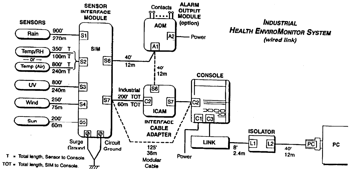
Figure 1c. Health EnviroMonitor System Schematic.
