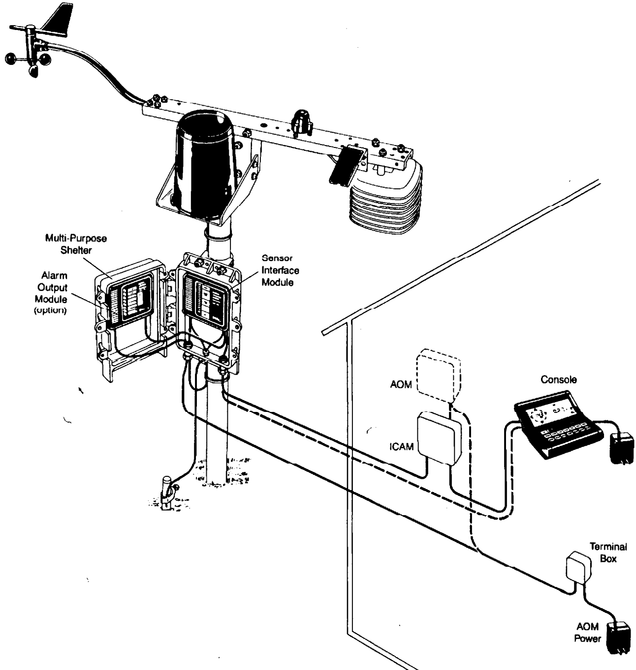
Figure 2. Field Interface System
